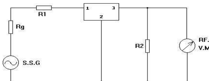
Rg+R1=R2=Input/Output Impedance
